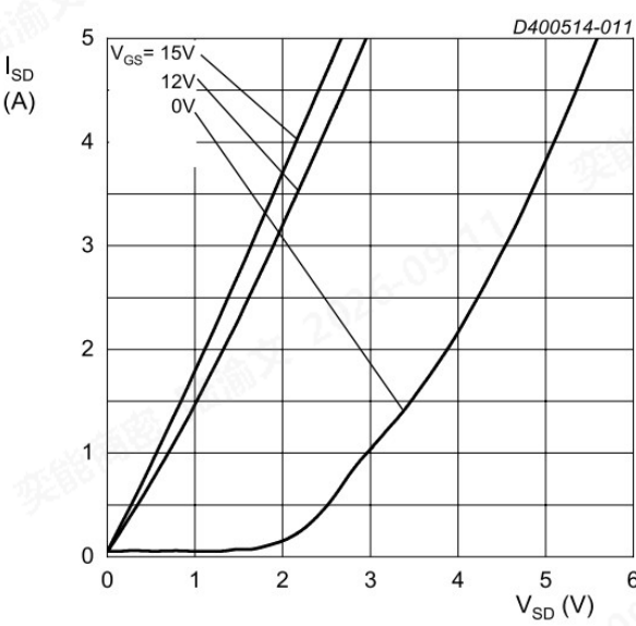
Figure 11 Body diode forward characteristics; typical values T_j = 25^\circ C ; t_p < 200\mu s
