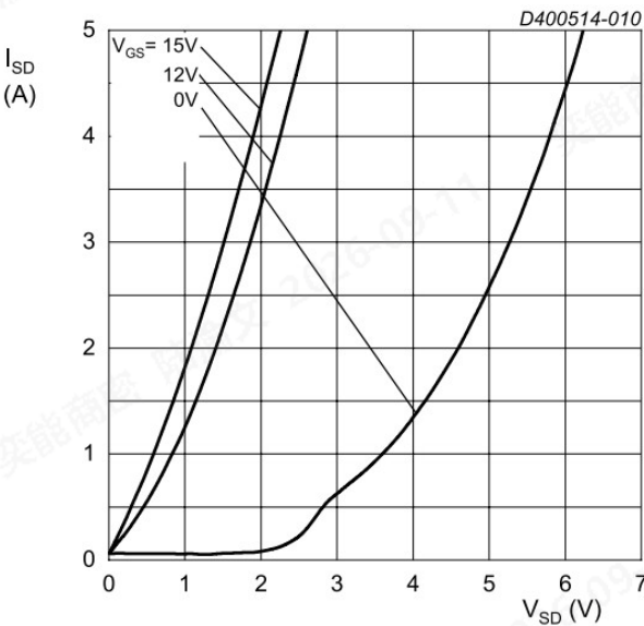
Figure 10 Body diode forward characteristics; typical values T_j = -55^\circ C ; t_p < 200\mu s
